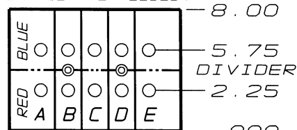
MANIFOLD HOLE PATTERN TOP VIEW (UNFOLDED)
